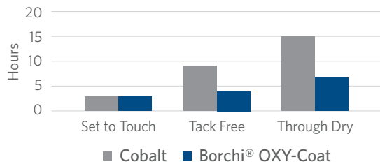
Standard Dry Time @ 23°C 50% RH Long Oil Alkyd
