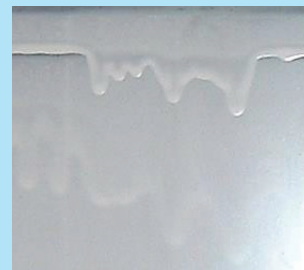
Figure 3a Spraying varnish for industrial coatings showing 'curtains'
